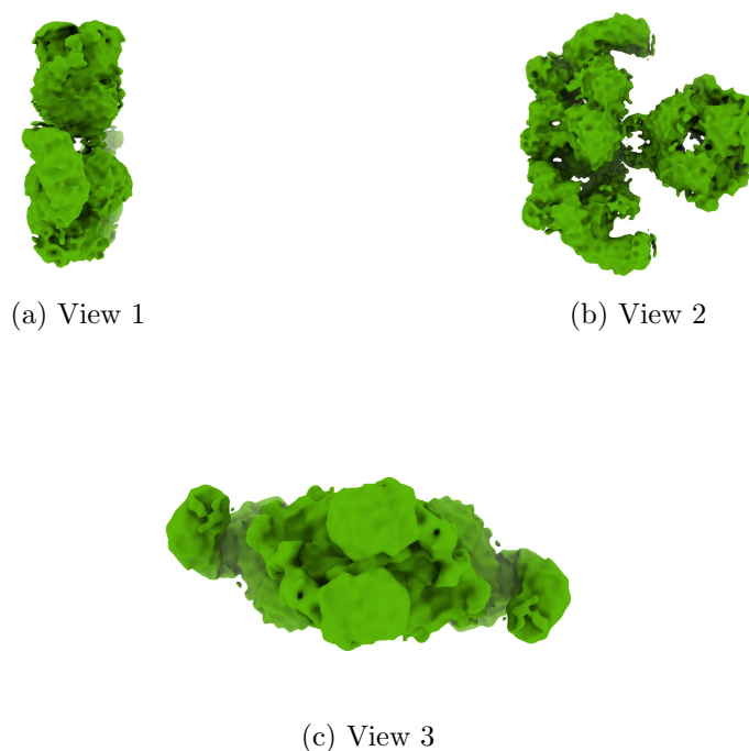
Figure 4: Isosurface at threshold=0.010500. Views generated by ChimeraX at a the following X, Y, Z angles: View 1 (0, -90, -90), View 2 (-90, 0, -90), View 3 (0, 0, 0).
