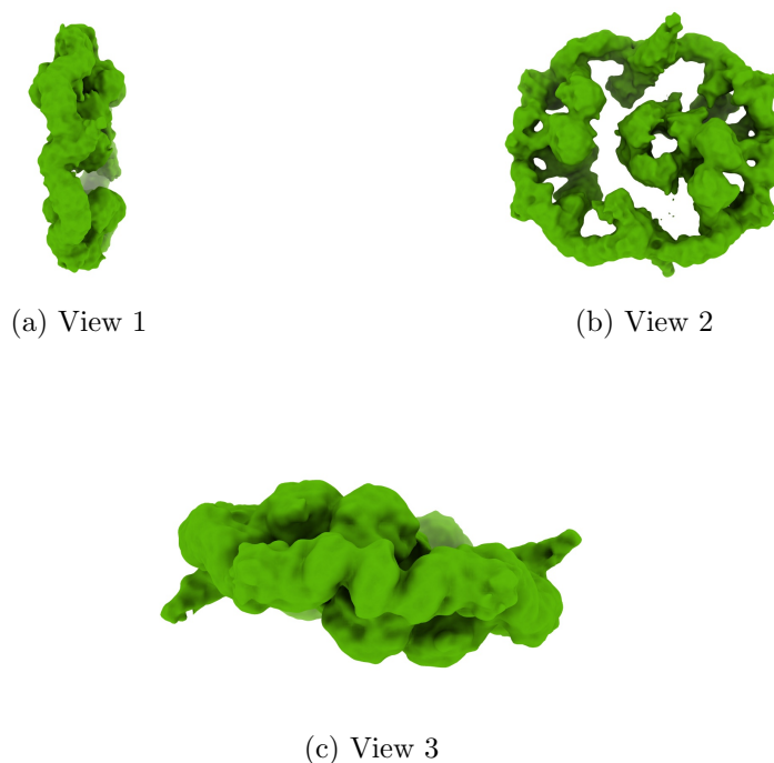
Figure 4: Isosurface at threshold=0.015100. Views generated by ChimeraX at a the following X, Y, Z angles: View 1 (0, -90, -90), View 2 (-90, 0, -90), View 3 (0, 0, 0).
