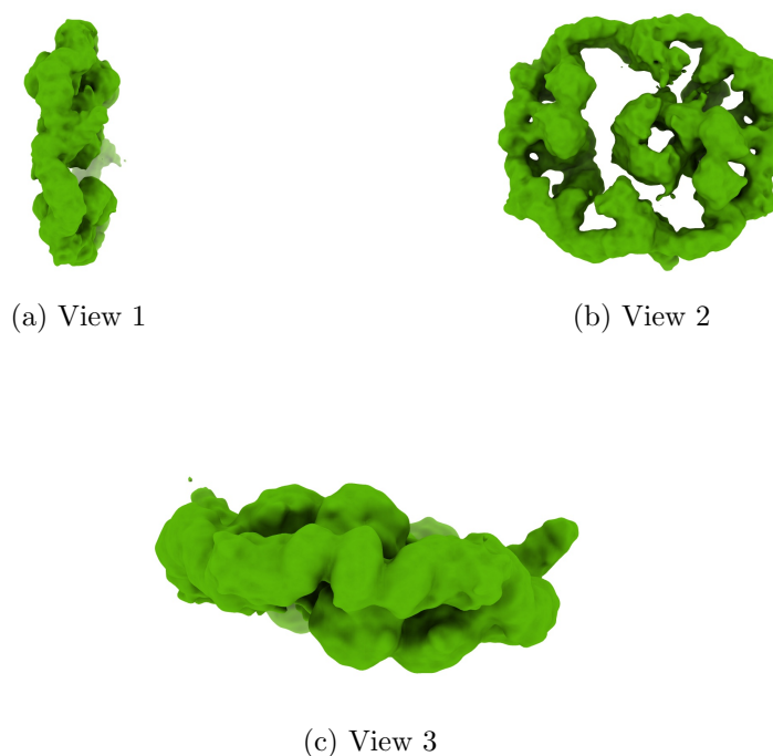
Figure 4: Isosurface at threshold=0.013400. Views generated by ChimeraX at a the following X, Y, Z angles: View 1 (0, -90, -90), View 2 (-90, 0, -90), View 3 (0, 0, 0).
