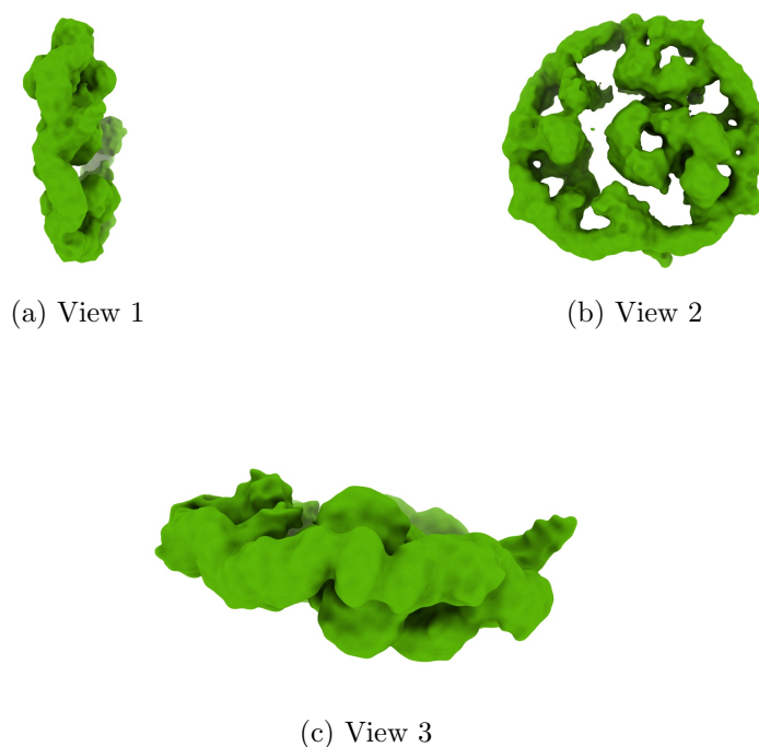
Figure 4: Isosurface at threshold=0.013700. Views generated by ChimeraX at a the following X, Y, Z angles: View 1 (0, -90, -90), View 2 (-90, 0, -90), View 3 (0, 0, 0).
