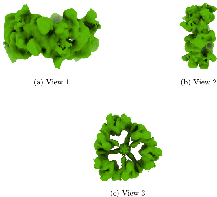
Figure 4: Isosurface at threshold=0.019500. Views generated by ChimeraX at a the following X, Y, Z angles: View 1 (0, -90, -90), View 2 (-90, 0, -90), View 3 (0, 0, 0).
