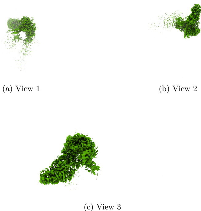
Figure 4: Isosurface at threshold=0.380000. Views generated by ChimeraX at a the following X, Y, Z angles: View 1 (0, -90, -90), View 2 (-90, 0, -90), View 3 (0, 0, 0).
