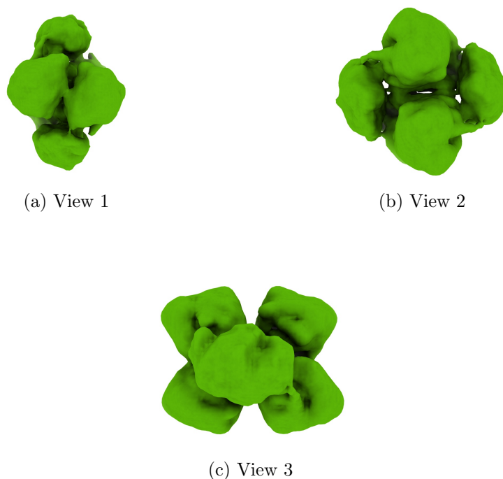
Figure 4: Isosurface at threshold=0.096100. Views generated by ChimeraX at a the following X, Y, Z angles: View 1 (0, -90, -90), View 2 (-90, 0, -90), View 3 (0, 0, 0).
