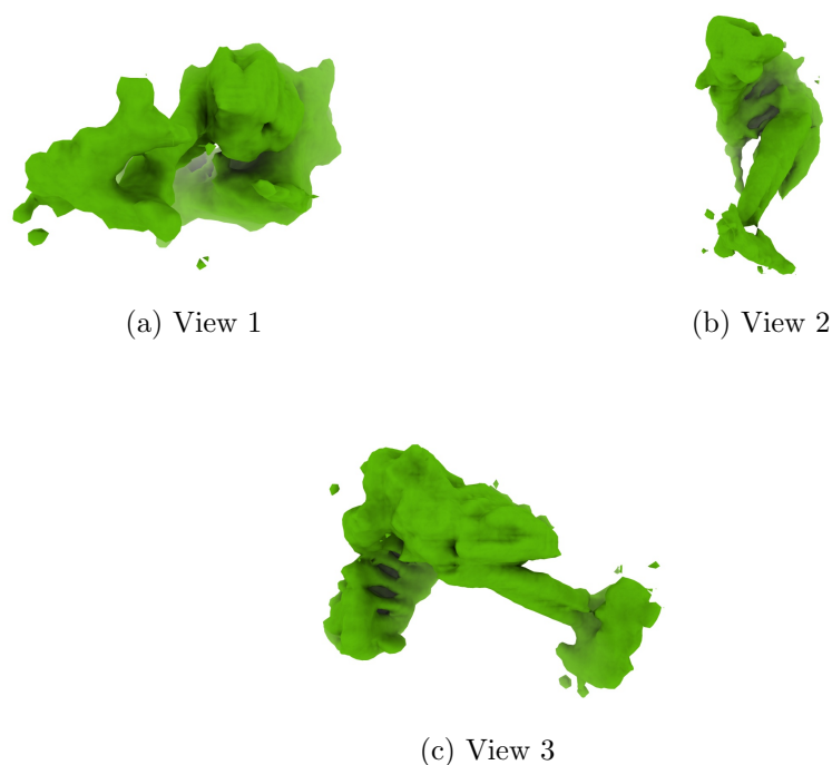
Figure 4: Isosurface at threshold=0.009080. Views generated by ChimeraX at a the following X, Y, Z angles: View 1 (0, -90, -90), View 2 (-90, 0, -90), View 3 (0, 0, 0).
