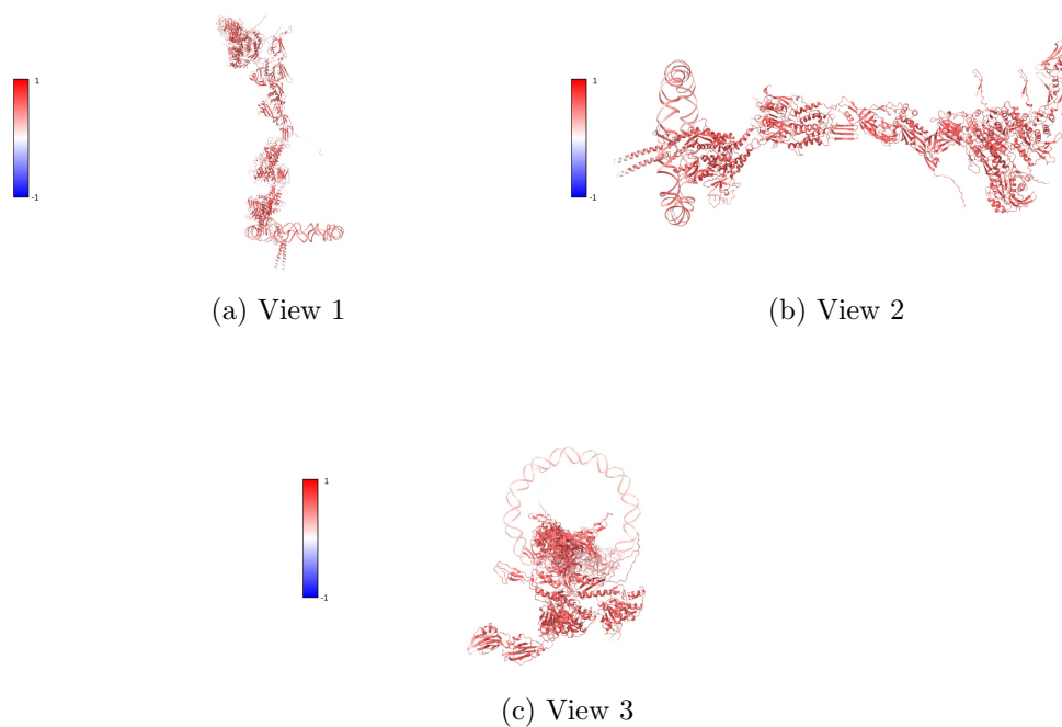
Figure 17: Atomic model colored by MapQ Views generated by ChimeraX at a the following X, Y, Z angles: View 1 (0, -90, -90), View 2 (-90, 0, -90), View 3 (0, 0, 0).
