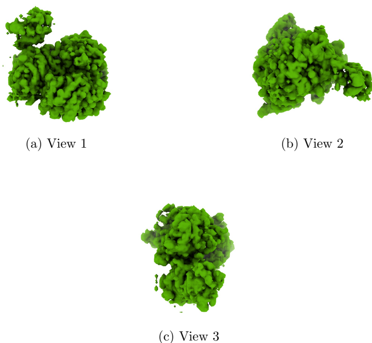
Figure 4: Isosurface at threshold=0.011700. Views generated by ChimeraX at a the following X, Y, Z angles: View 1 (0, -90, -90), View 2 (-90, 0, -90), View 3 (0, 0, 0).
