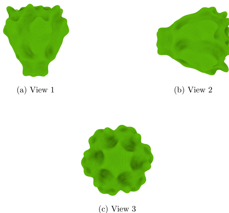
Figure 4: Isosurface at threshold=0.861000. Views generated by ChimeraX at a the following X, Y, Z angles: View 1 (0, -90, -90), View 2 (-90, 0, -90), View 3 (0, 0, 0).
