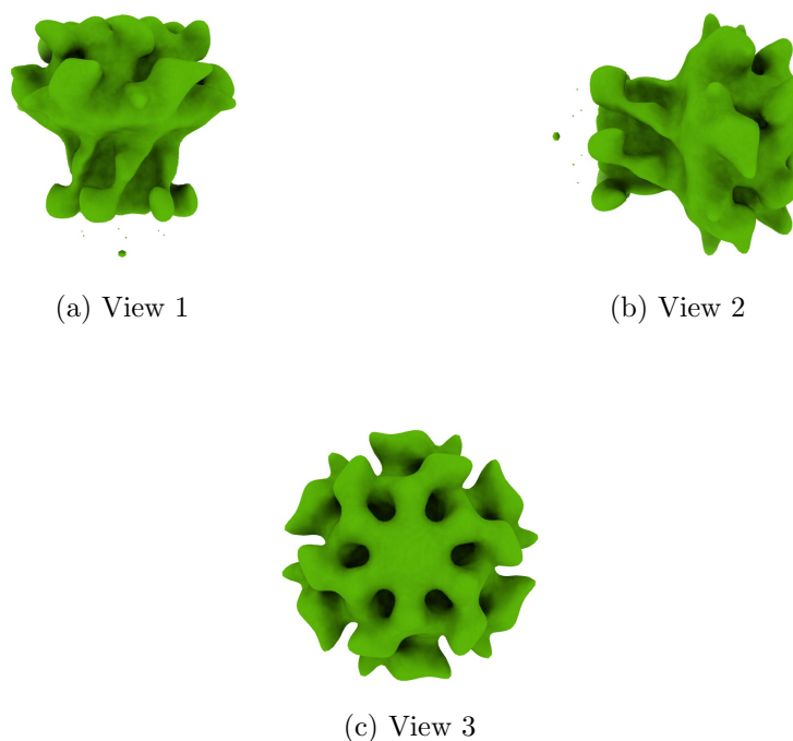
Figure 4: Isosurface at threshold=1.060000. Views generated by ChimeraX at a the following X, Y, Z angles: View 1 (0, -90, -90), View 2 (-90, 0, -90), View 3 (0, 0, 0).
