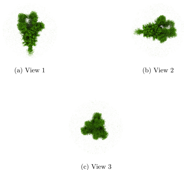
Figure 4: Isosurface at threshold=0.094300. Views generated by ChimeraX at a the following X, Y, Z angles: View 1 (0, -90, -90), View 2 (-90, 0, -90), View 3 (0, 0, 0).
