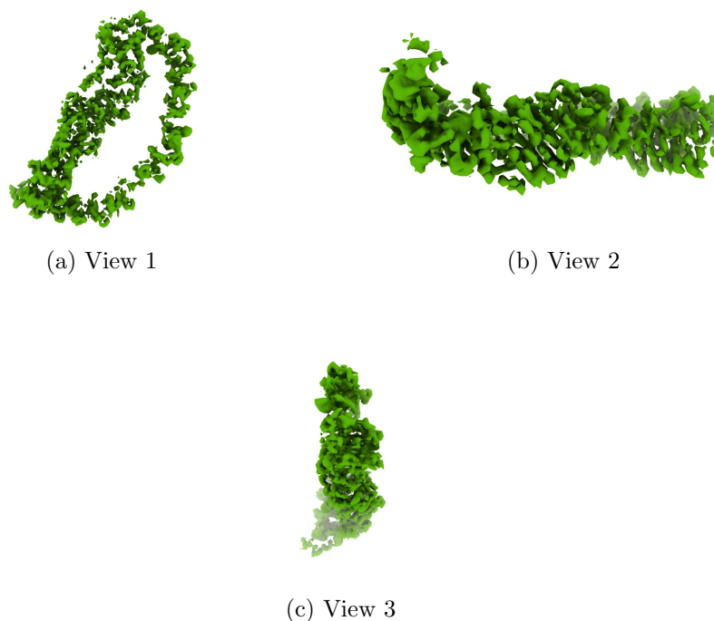
Figure 4: Isosurface at threshold=0.331000. Views generated by ChimeraX at the following X, Y, Z angles: View 1 (0, -90, -90), View 2 (-90, 0, -90), View 3 (0, 0, 0).
