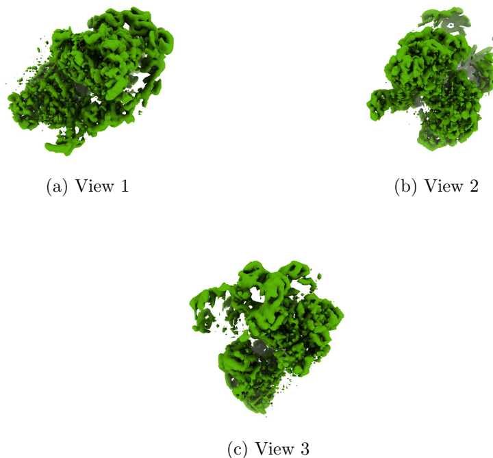
Figure 4: Isosurface at threshold=0.187000. Views generated by ChimeraX at a the following X, Y, Z angles: View 1 (0, -90, -90), View 2 (-90, 0, -90), View 3 (0, 0, 0).
