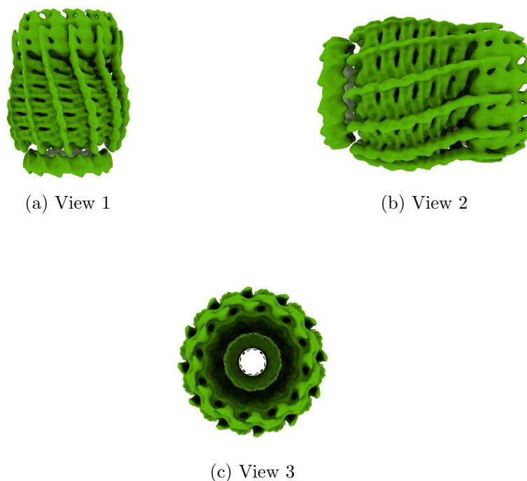
Figure 4: Isosurface at threshold=0.095400. Views generated by ChimeraX at a the following X, Y, Z angles: View 1 (0, -90, -90), View 2 (-90, 0, -90), View 3 (0, 0, 0).
