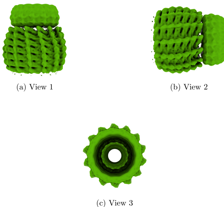
Figure 4: Isosurface at threshold=0.080500. Views generated by ChimeraX at a the following X, Y, Z angles: View 1 (0, -90, -90), View 2 (-90, 0, -90), View 3 (0, 0, 0).
