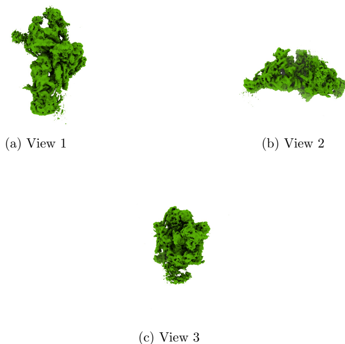
Figure 4: Isosurface at threshold=0.125000. Views generated by ChimeraX at a the following X, Y, Z angles: View 1 (0, -90, -90), View 2 (-90, 0, -90), View 3 (0, 0, 0).
