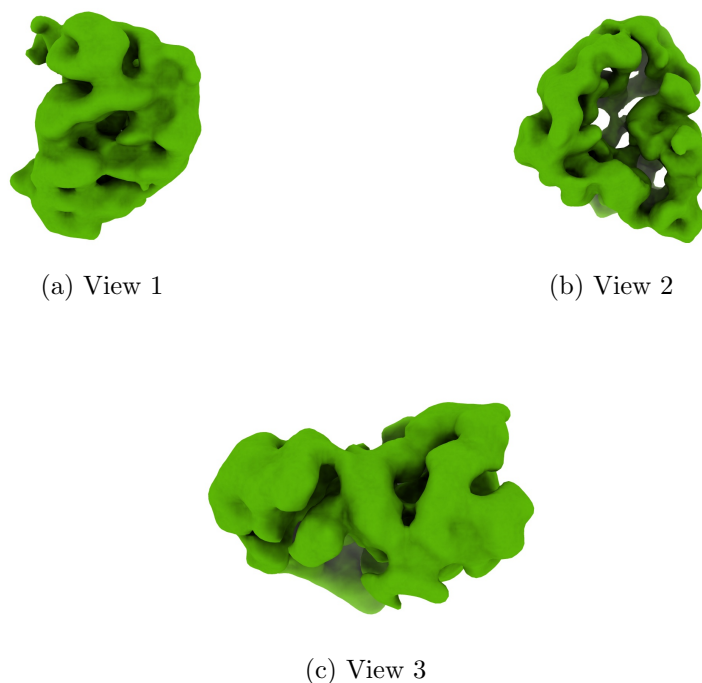
Figure 4: Isosurface at threshold=8.800000. Views generated by ChimeraX at a the following X, Y, Z angles: View 1 (0, -90, -90), View 2 (-90, 0, -90), View 3 (0, 0, 0).
