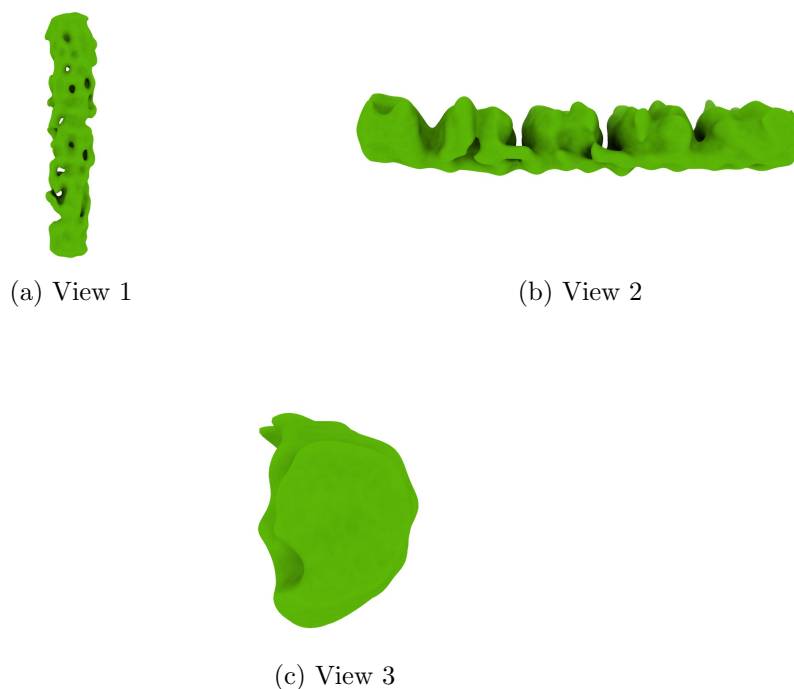
Figure 4: Isosurface at threshold=1.200000. Views generated by ChimeraX at a the following X, Y, Z angles: View 1 (0, -90, -90), View 2 (-90, 0, -90), View 3 (0, 0, 0).
