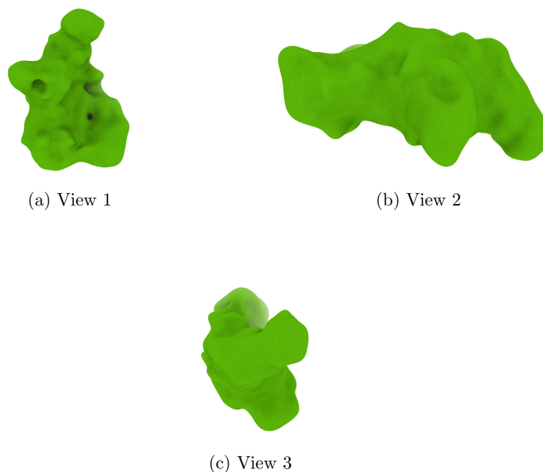
Figure 4: Isosurface at threshold=0.025500. Views generated by ChimeraX at a the following X, Y, Z angles: View 1 (0, -90, -90), View 2 (-90, 0, -90), View 3 (0, 0, 0).
