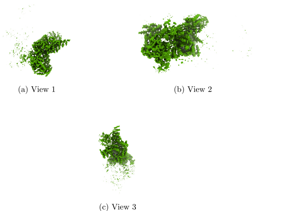
Figure 4: Isosurface at threshold=0.300000. Views generated by ChimeraX at a the following X, Y, Z angles: View 1 (0, -90, -90), View 2 (-90, 0, -90), View 3 (0, 0, 0).
