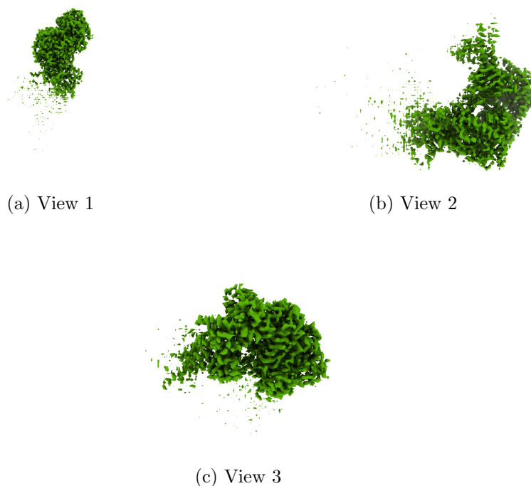
Figure 4: Isosurface at threshold=0.480000. Views generated by ChimeraX at a the following X, Y, Z angles: View 1 (0, -90, -90), View 2 (-90, 0, -90), View 3 (0, 0, 0).
