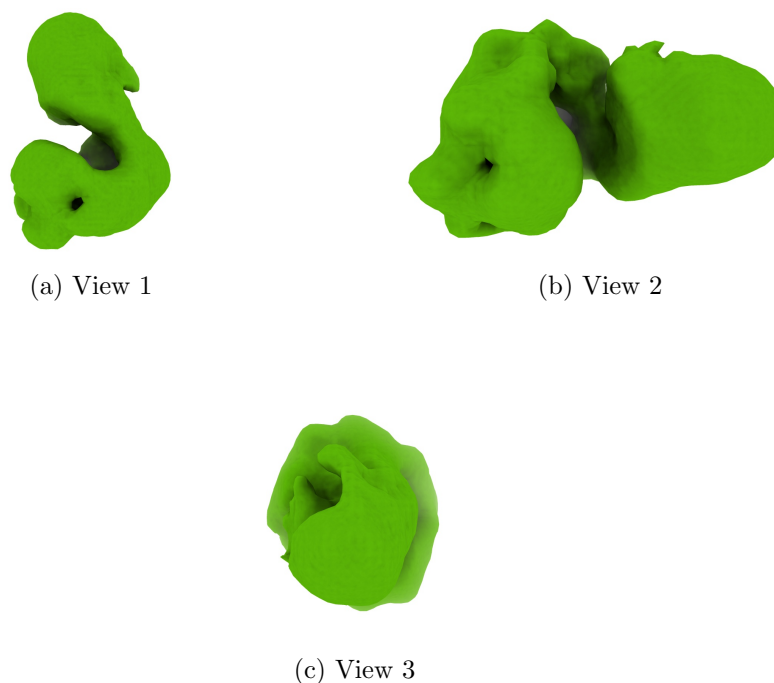
Figure 4: Isosurface at threshold=0.056000. Views generated by ChimeraX at a the following X, Y, Z angles: View 1 (0, -90, -90), View 2 (-90, 0, -90), View 3 (0, 0, 0).
