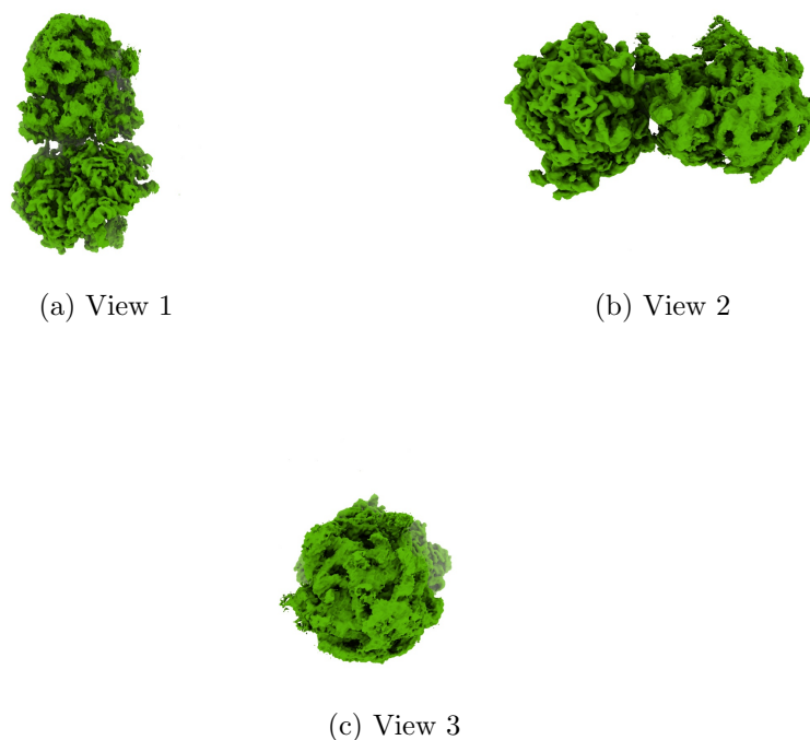
Figure 4: Isosurface at threshold=0.275000. Views generated by ChimeraX at a the following X, Y, Z angles: View 1 (0, -90, -90), View 2 (-90, 0, -90), View 3 (0, 0, 0).
