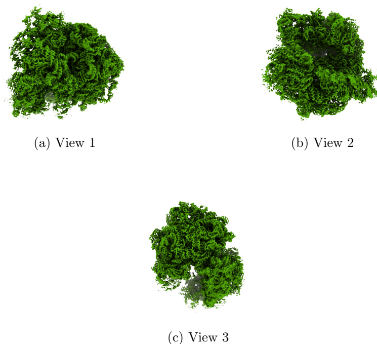
Figure 4: Isosurface at threshold=0.009380. Views generated by ChimeraX at a the following X, Y, Z angles: View 1 (0, -90, -90), View 2 (-90, 0, -90), View 3 (0, 0, 0).
