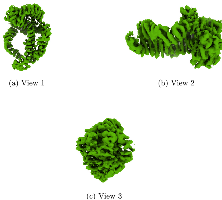
Figure 4: Isosurface at threshold=0.112000. Views generated by ChimeraX at a the following X, Y, Z angles: View 1 (0, -90, -90), View 2 (-90, 0, -90), View 3 (0, 0, 0).
