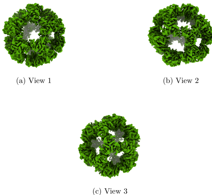
Figure 4: Isosurface at threshold=0.650000. Views generated by ChimeraX at the following X, Y, Z angles: View 1 (0, -90, -90), View 2 (-90, 0, -90), View 3 (0, 0, 0).
