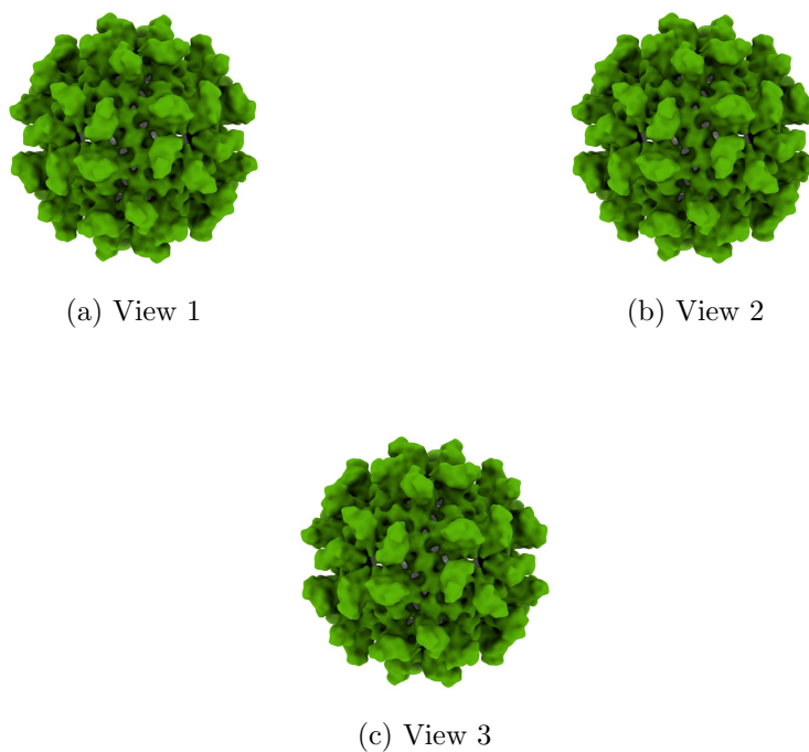
Figure 4: Isosurface at threshold=297.000000. Views generated by ChimeraX at a the following X, Y, Z angles: View 1 (0, -90, -90), View 2 (-90, 0, -90), View 3 (0, 0, 0).
