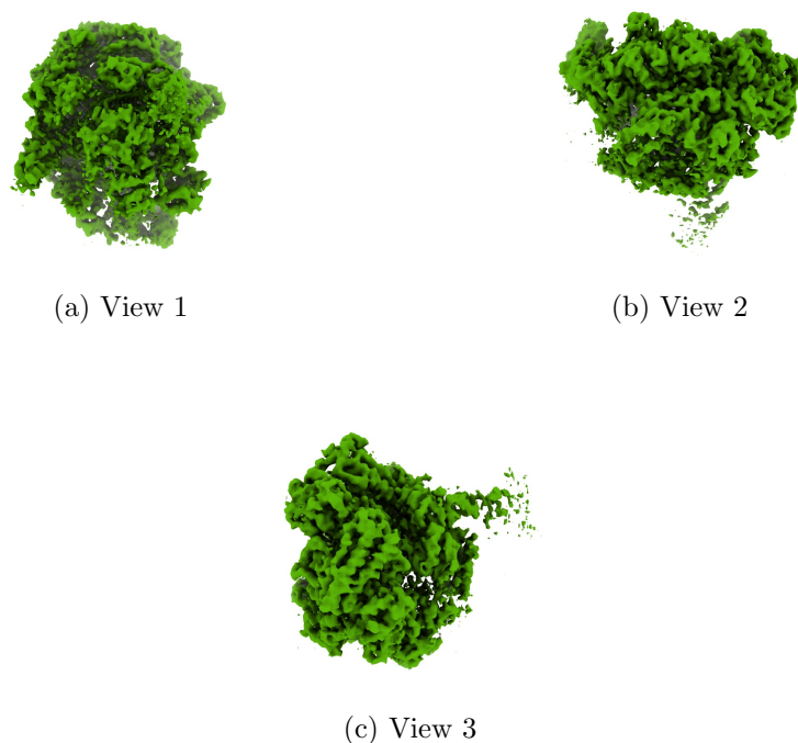
Figure 4: Isosurface at threshold=0.078300. Views generated by ChimeraX at a the following X, Y, Z angles: View 1 (0, -90, -90), View 2 (-90, 0, -90), View 3 (0, 0, 0).
