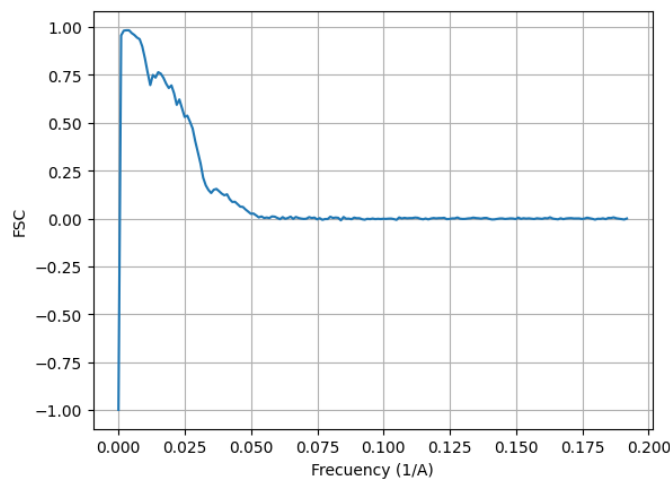
Figure 20: FSC and resolution estimated by a permutation test.
