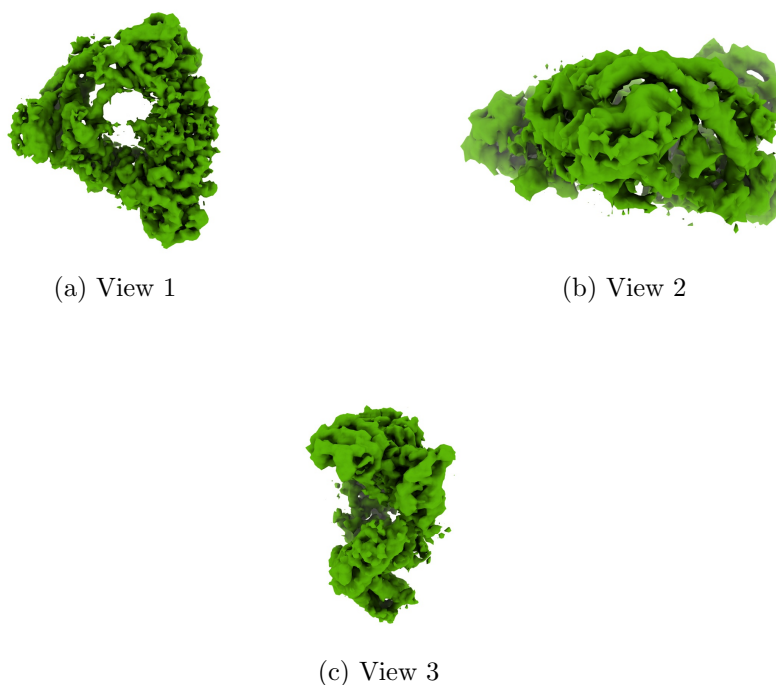
Figure 4: Isosurface at threshold=0.077600. Views generated by ChimeraX at a the following X, Y, Z angles: View 1 (0, -90, -90), View 2 (-90, 0, -90), View 3 (0, 0, 0).
