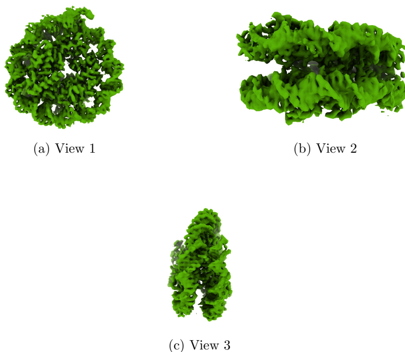
Figure 4: Isosurface at threshold=0.263000. Views generated by ChimeraX at a the following X, Y, Z angles: View 1 (0, -90, -90), View 2 (-90, 0, -90), View 3 (0, 0, 0).
