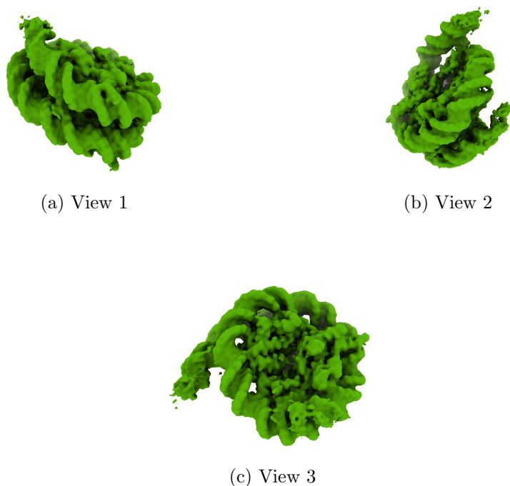
Figure 4: Isosurface at threshold=0.082500. Views generated by ChimeraX at a the following X, Y, Z angles: View 1 (0, -90, -90), View 2 (-90, 0, -90), View 3 (0, 0, 0).
