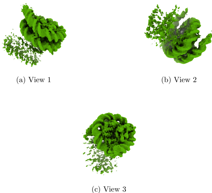
Figure 4: Isosurface at threshold=0.085200. Views generated by ChimeraX at a the following X, Y, Z angles: View 1 (0, -90, -90), View 2 (-90, 0, -90), View 3 (0, 0, 0).
