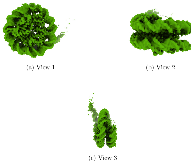
Figure 4: Isosurface at threshold=0.080300. Views generated by ChimeraX at a the following X, Y, Z angles: View 1 (0, -90, -90), View 2 (-90, 0, -90), View 3 (0, 0, 0).
