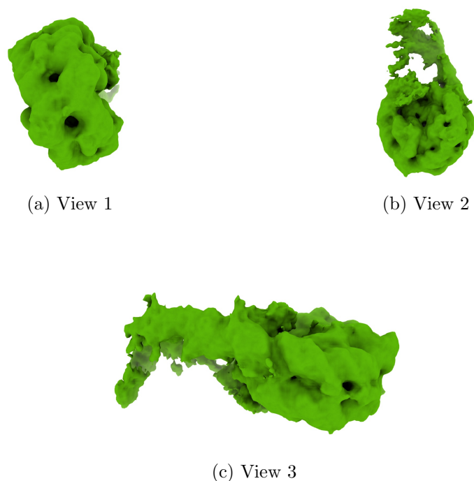
Figure 4: Isosurface at threshold=0.006380. Views generated by ChimeraX at a the following X, Y, Z angles: View 1 (0, -90, -90), View 2 (-90, 0, -90), View 3 (0, 0, 0).
