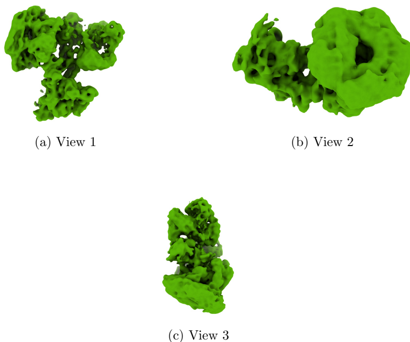
Figure 4: Isosurface at threshold=0.850000. Views generated by ChimeraX at a the following X, Y, Z angles: View 1 (0, -90, -90), View 2 (-90, 0, -90), View 3 (0, 0, 0).
