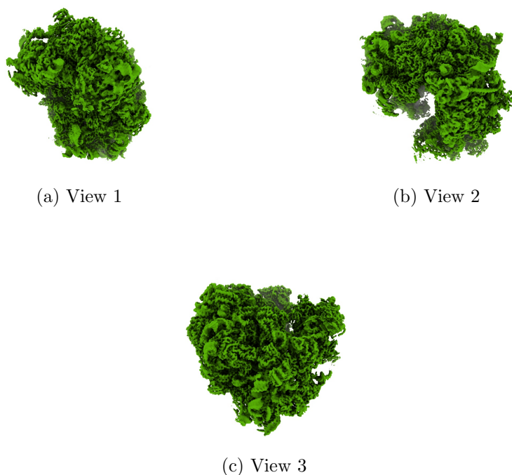
Figure 4: Isosurface at threshold=0.007610. Views generated by ChimeraX at a the following X, Y, Z angles: View 1 (0, -90, -90), View 2 (-90, 0, -90), View 3 (0, 0, 0).
