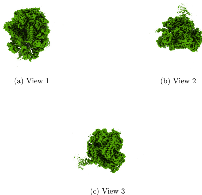
Figure 4: Isosurface at threshold=0.093700. Views generated by ChimeraX at a the following X, Y, Z angles: View 1 (0, -90, -90), View 2 (-90, 0, -90), View 3 (0, 0, 0).
