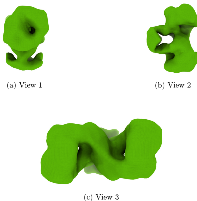
Figure 4: Isosurface at threshold=0.430000. Views generated by ChimeraX at a the following X, Y, Z angles: View 1 (0, -90, -90), View 2 (-90, 0, -90), View 3 (0, 0, 0).
