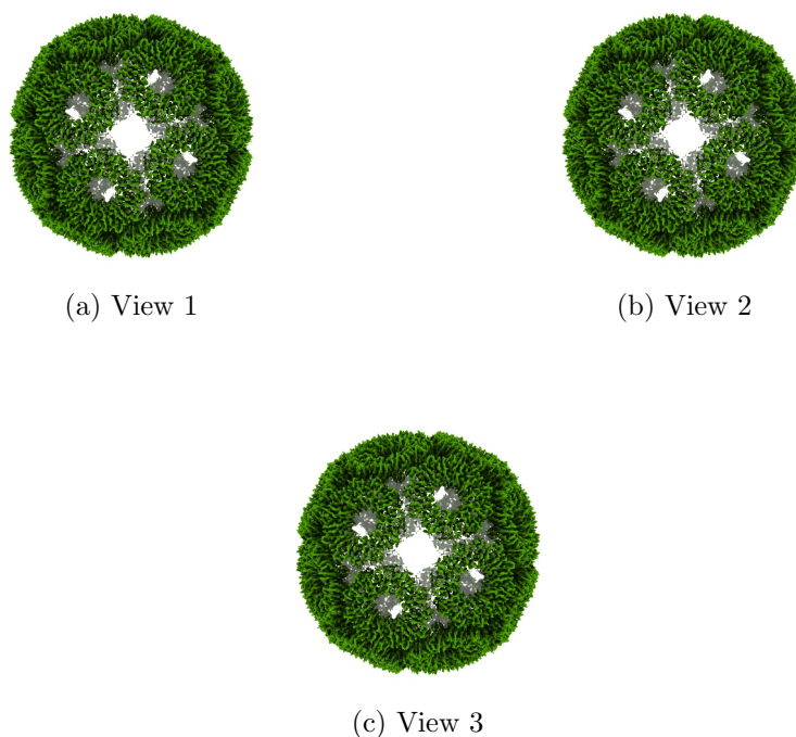
Figure 4: Isosurface at threshold=0.243000. Views generated by ChimeraX at a the following X, Y, Z angles: View 1 (0, -90, -90), View 2 (-90, 0, -90), View 3 (0, 0, 0).
