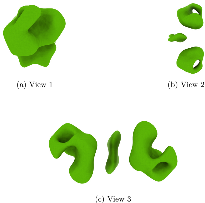
Figure 4: Isosurface at threshold=3.920000. Views generated by ChimeraX at a the following X, Y, Z angles: View 1 (0, -90, -90), View 2 (-90, 0, -90), View 3 (0, 0, 0).
