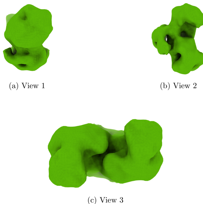
Figure 4: Isosurface at threshold=3.200000. Views generated by ChimeraX at a the following X, Y, Z angles: View 1 (0, -90, -90), View 2 (-90, 0, -90), View 3 (0, 0, 0).
