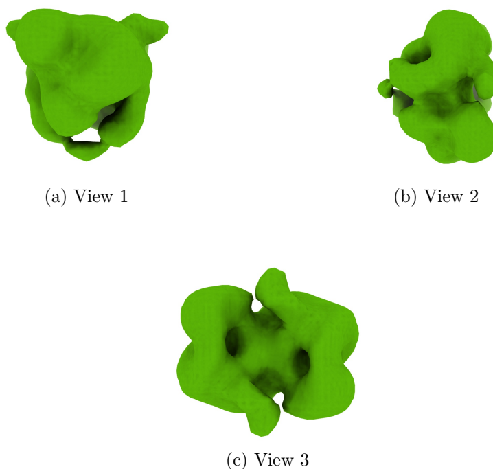
Figure 4: Isosurface at threshold=2.100000. Views generated by ChimeraX at a the following X, Y, Z angles: View 1 (0, -90, -90), View 2 (-90, 0, -90), View 3 (0, 0, 0).
