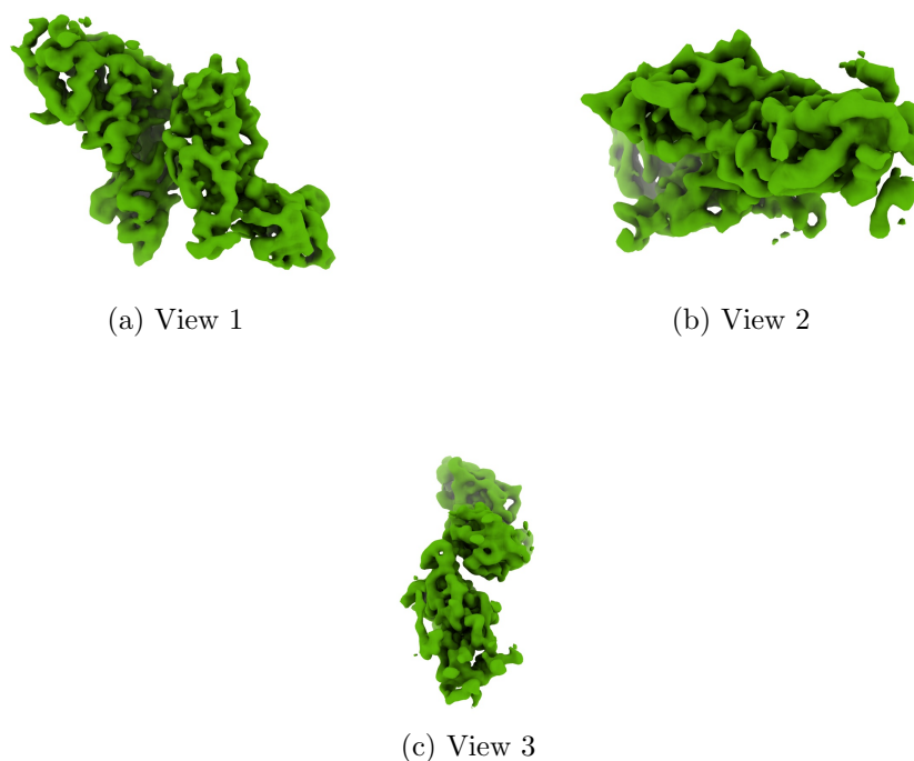
Figure 4: Isosurface at threshold=0.033000. Views generated by ChimeraX at a the following X, Y, Z angles: View 1 (0, -90, -90), View 2 (-90, 0, -90), View 3 (0, 0, 0).
