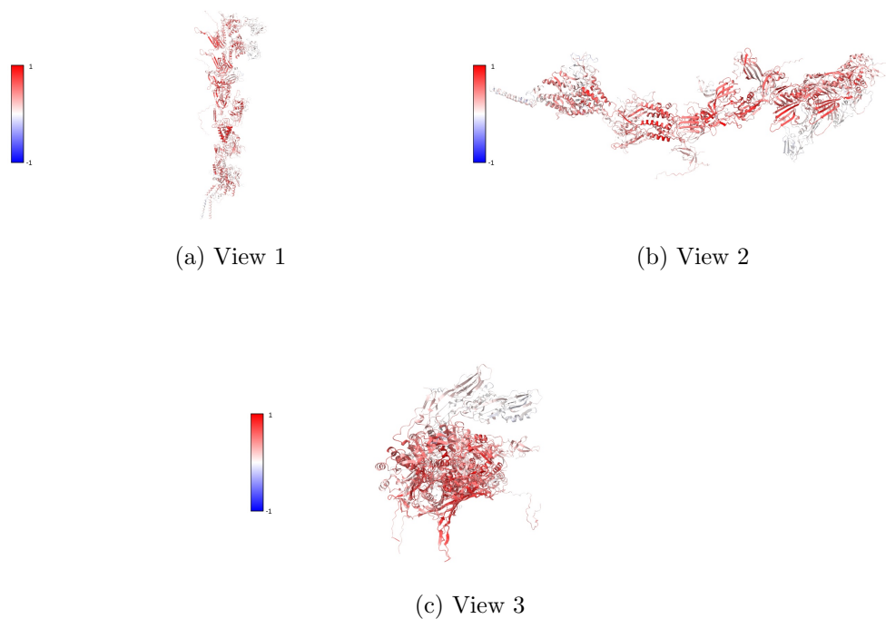
Figure 19: Atomic model colored by DAQ Views generated by ChimeraX at the following X, Y, Z angles: View 1 (0, -90, -90), View 2 (-90, 0, -90), View 3 (0, 0, 0).
