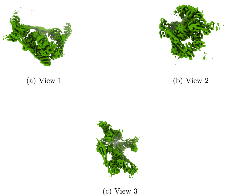
Figure 4: Isosurface at threshold=0.735000. Views generated by ChimeraX at a the following X, Y, Z angles: View 1 (0, -90, -90), View 2 (-90, 0, -90), View 3 (0, 0, 0).
