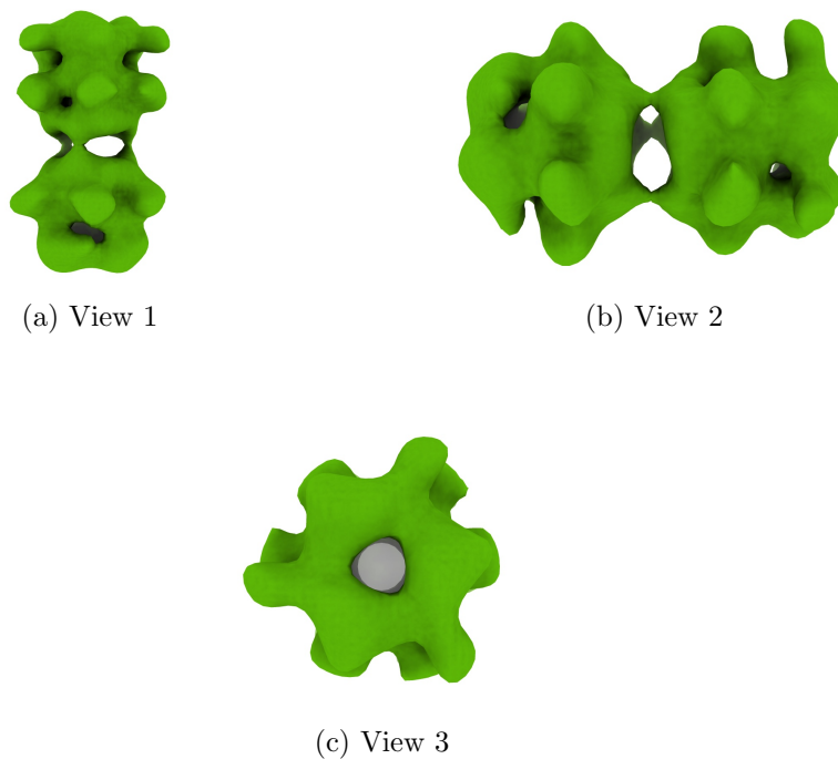
Figure 4: Isosurface at threshold=60.000000. Views generated by ChimeraX at a the following X, Y, Z angles: View 1 (0, -90, -90), View 2 (-90, 0, -90), View 3 (0, 0, 0).
