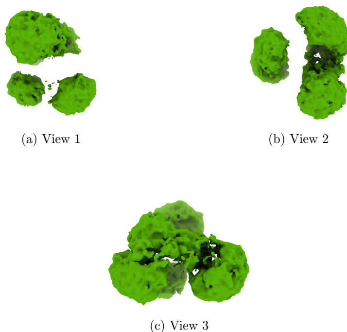
Figure 4: Isosurface at threshold=0.893000. Views generated by ChimeraX at a the following X, Y, Z angles: View 1 (0, -90, -90), View 2 (-90, 0, -90), View 3 (0, 0, 0).
